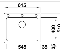
Cut out size: 595 x 490 x R15
