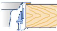
Stainless steel: Installation from above, flat lay-on
